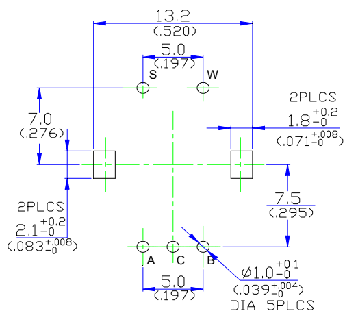
MOUNTING HOLE DETAILS DIMENSIONS: MM (INCHES)
