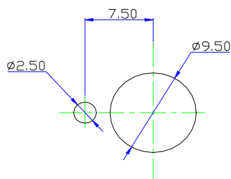
MOUNTING HOLE DETAILS
